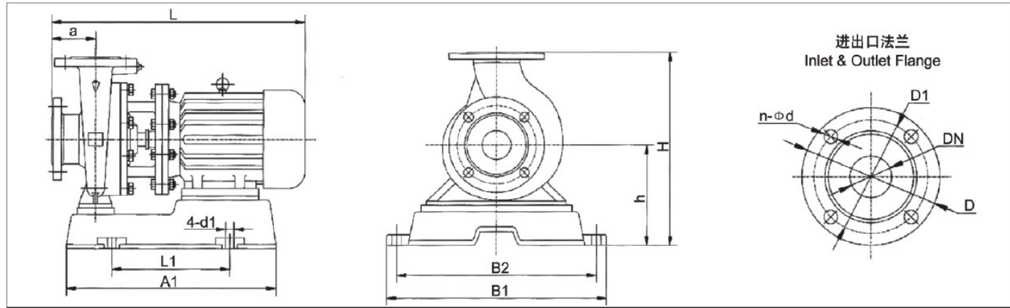
ISW 型泵性能参数表、安装尺寸图及安装尺寸表 Performance Parameters Table, Installation Dimensions Drawing and Installation Dimensions Table of SCW Pumps
