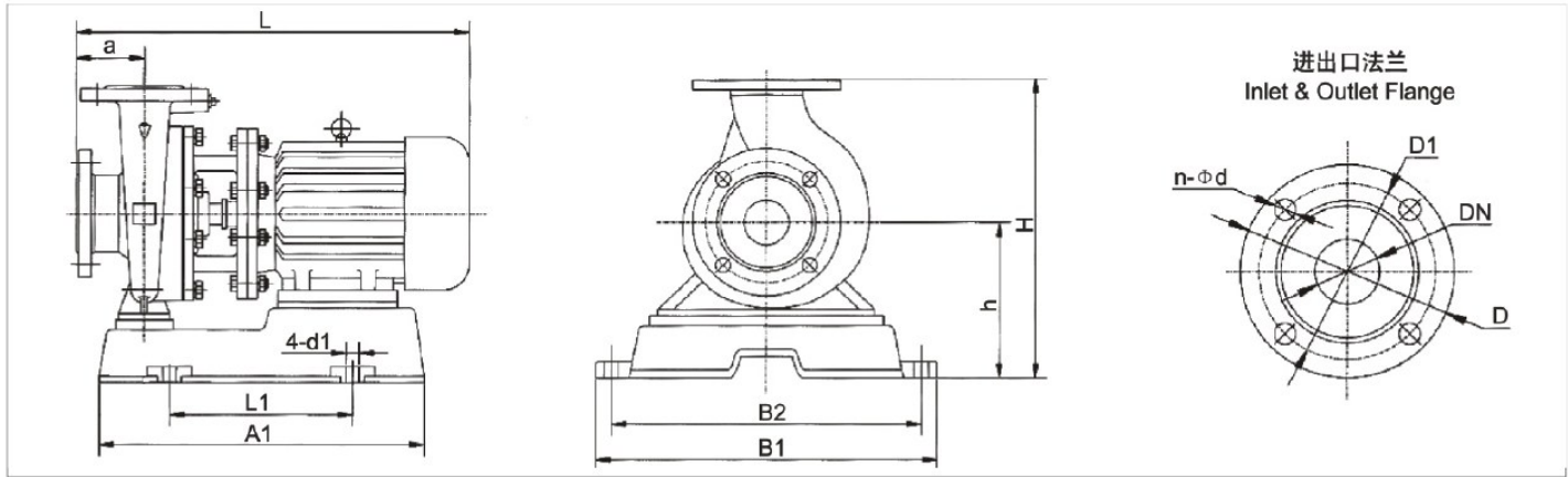
型泵性能参数表、安装尺寸图及安装尺寸表 Performance Parameters Table, Installation Dimensions Drawing and Installation Dimensions Table of SCW Pumps
